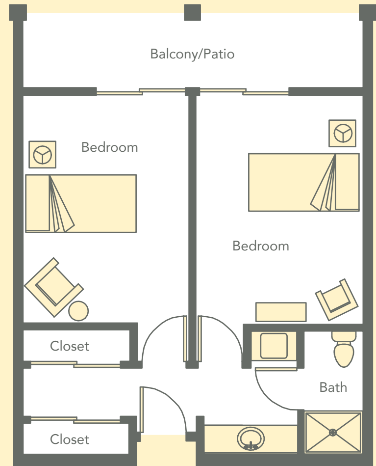
Assisted Living Side-by-Side (570 Sq. Ft.)
